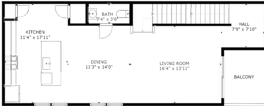
FLOOR 2
